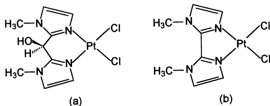
Fig. 9. Structures of the (a) anti-cancer active [PtCl 2 (bmic)] and (b) inactive [PtCl 2 (bmi)].
